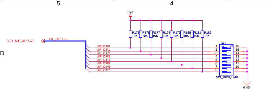
User switches
