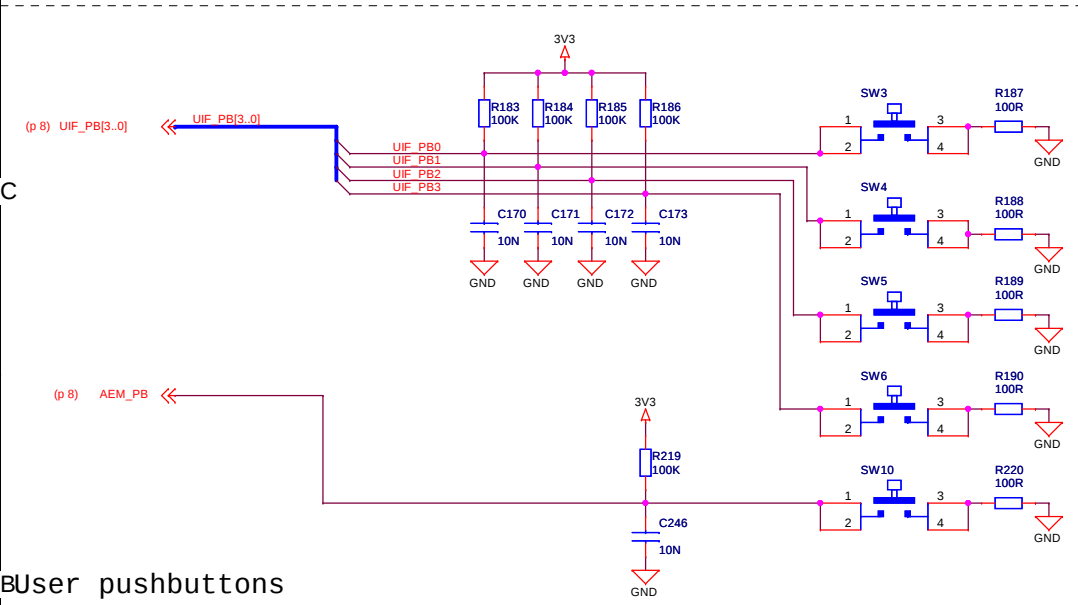
User pushbuttons
